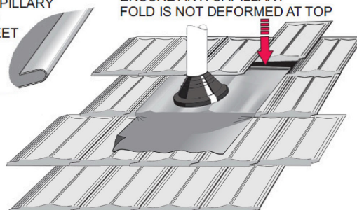
ENSURE ANTI CAPILLARY FOLD IS NOT DEFORMED AT TOP
