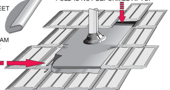
ENSURE ANTI CAPILLARY FOLD IS NOT DEFORMED AT TOP
